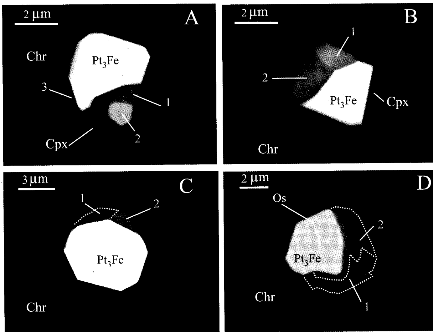
FIG. 6. BSE images of primary composite grains included in chromian spinel (Chr) from the Kytlym chromitites, showing isoferroplatinum-type alloys ( Pt_3Fe ) overgrown by various sulfides and clinopyroxene (not ubiquitous). A) Grain KT349B-2a, unknown PGE-bearing base-metal monosulfide ( Fe_{0.27}Ni_{0.22}Cu_{0.08}S_{2.04} ) \Sigma_{0.57}(Rh_{0.17}Ir_{0.08}Os_{0.08}Pt_{0.04})\Sigma_{0.37}S_{1.06} (1), erlichmanite ( Os_{0.68}Ir_{0.04}Ru_{0.13}Ni_{0.09}Fe_{0.02}S_{2.04} ) \Sigma_{0.96}S_{2.04} (2), Fe-Ni sulfide, possibly pentlandite (3), and clinopyroxene (Cpx). B) Grain KT349B-4b, cuprorhodite ( Cu_{0.73}Fe_{0.27}Ni_{0.06}S_{1.06}(Rh_{0.75}Ir_{0.47}Pt_{0.68}Os_{0.07}Ru_{0.02})\Sigma_{1.99}S_{3.95} ) (1), unknown PGE-bearing base-metal monosulfide ( Fe_{0.27}Ni_{0.17}Cu_{0.12}S_{0.56}(Rh_{0.19}Ir_{0.1}Os_{0.05}Pt_{0.02}Pd_{0.02})\Sigma_{0.38}S_{1.06} ) (2), and clinopyroxene (Cpx). C) Grain KT349B-5a, pyrrhotite Fe_{0.96}Ni_{0.02}(Rh + Pt)_{0.02}S_{1.0} (1), and unknown PGE-bearing base-metal monosulfide ( Fe_{0.27}Ni_{0.23}Cu_{0.12}S_{0.62}(Rh_{0.23}Ir_{0.05}Pt_{0.06})\Sigma_{0.34}S_{1.04} ) (2). D) Grain KT349B-28b, pentlandite (1), and pyrrhotite (2). The grain contains one exsolution lamella of native osmium (Os).
