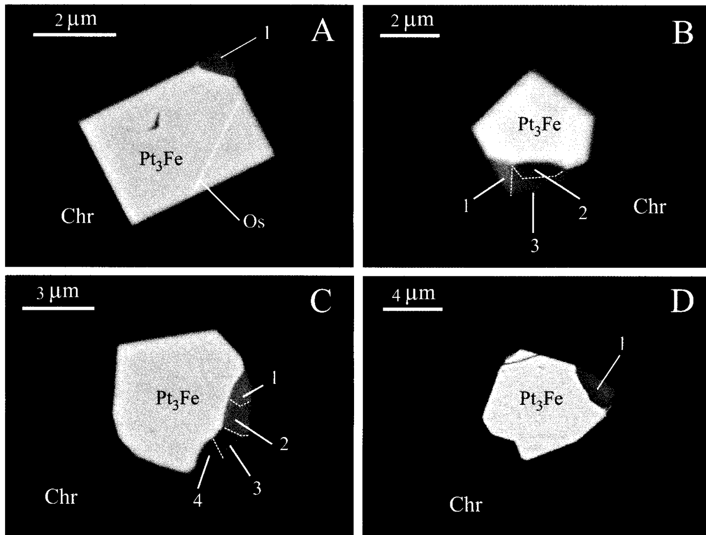
FIG. 5. BSE images of primary composite grains included in chromian spinel (Chr) from the Uktus chromitites, showing isoferroplatinum-type alloys ( Pt_3Fe ) overgrown by PGE sulfides. A) Grain UK296B–5, erlichmanite (1). Isoferroplatinum contains one thin exsolution lamella of native osmium (Os). B) Grain UK296B–16a, erlichmanite (1), cuprorhodsite (2) and cuproiridsite (3). C) Grain UK296A–1, erlichmanite (1), Ru-rich erlichmanite (2), cuproiridsite (3), and cuprorhodsite (4). D) Grain UK296A–12, cuprorhodsite ( Cu_{0.72}Ni_{0.08}Fe_{0.04})_{\Sigma 0.84}(Rh_{1.24}Ir_{0.81}Pt_{0.02})_{\Sigma 2.08}S_{4.08} .
